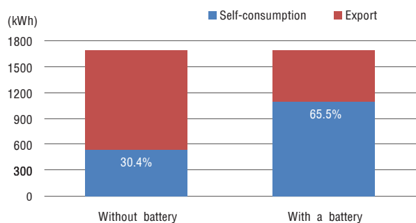
Self-consumption increased by 35.1% with 6.4 kWh battery Project 1 in Australia, Jan 2016
